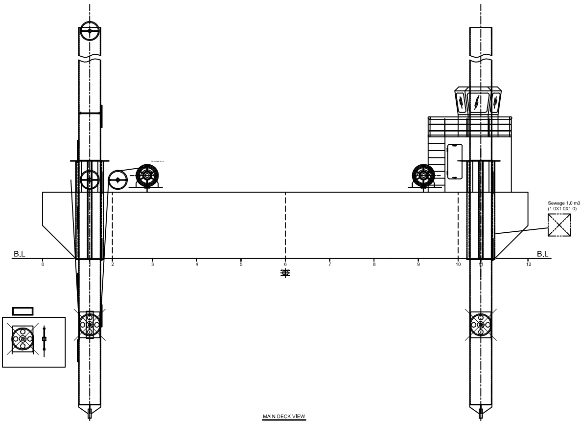
MAIN DECK VIEW
