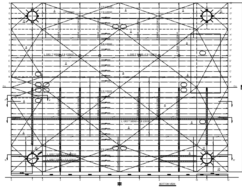
BOTTOM VIEW
