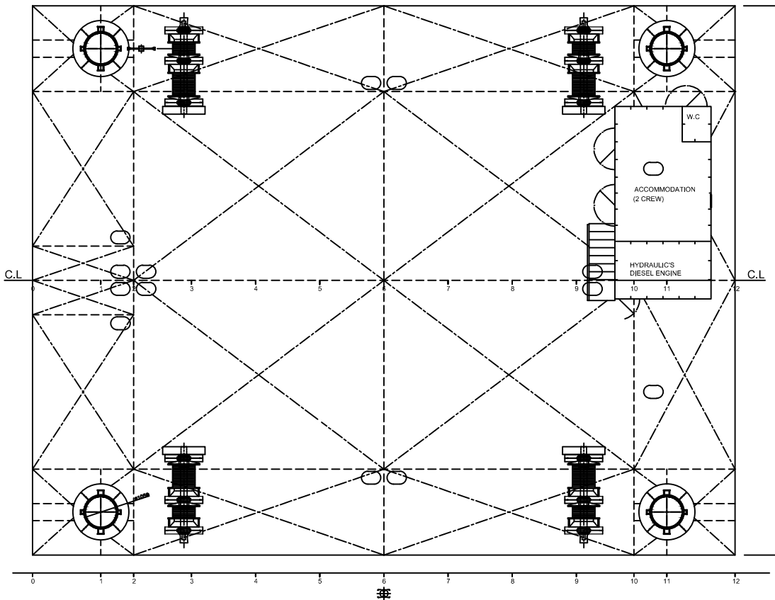
MAIN DECK VIEW
