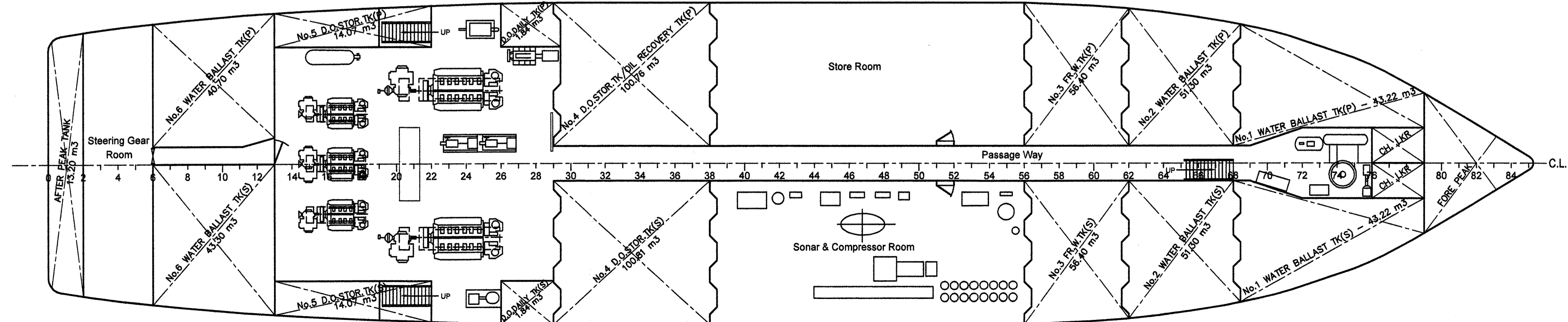
LOWER VIEW
