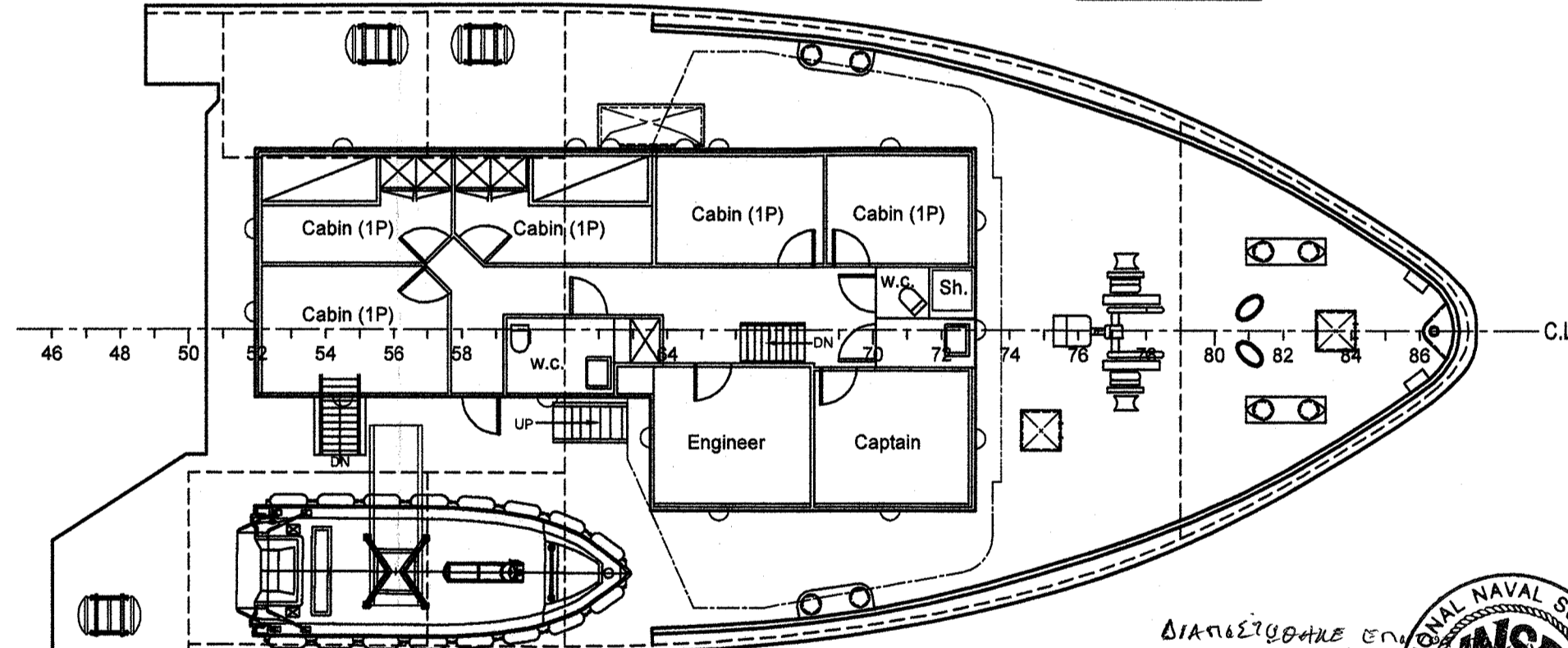
BOAT DECK
