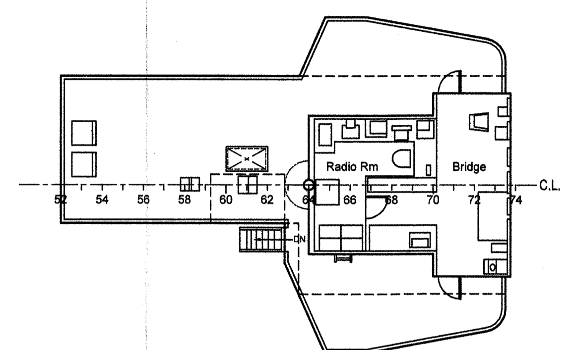
BRIDGE DECK
