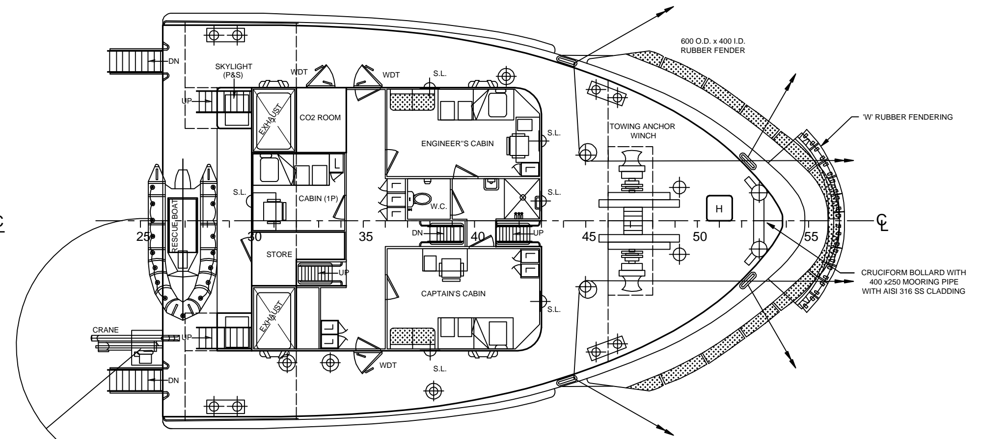
FORECASTLE DECK
