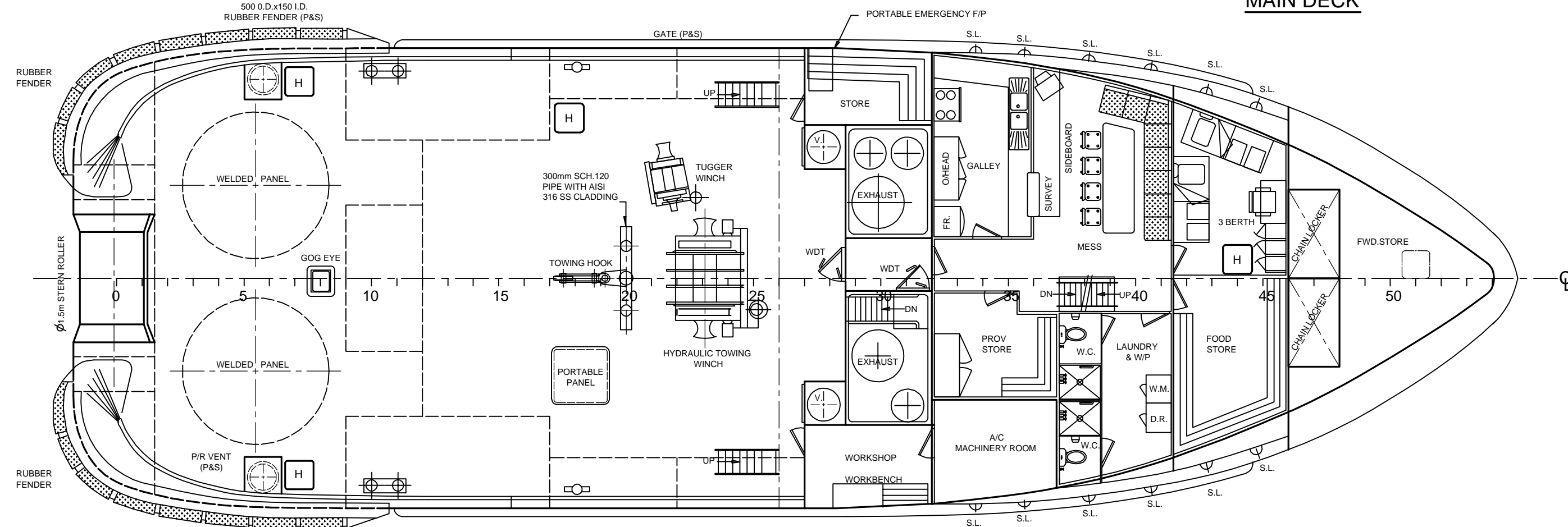
MAIN DECK
